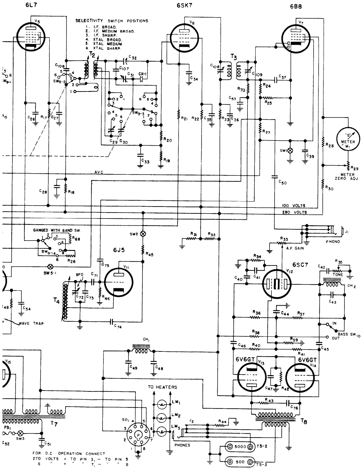
FIG. 13-SX28-A-SCHEMATIC
