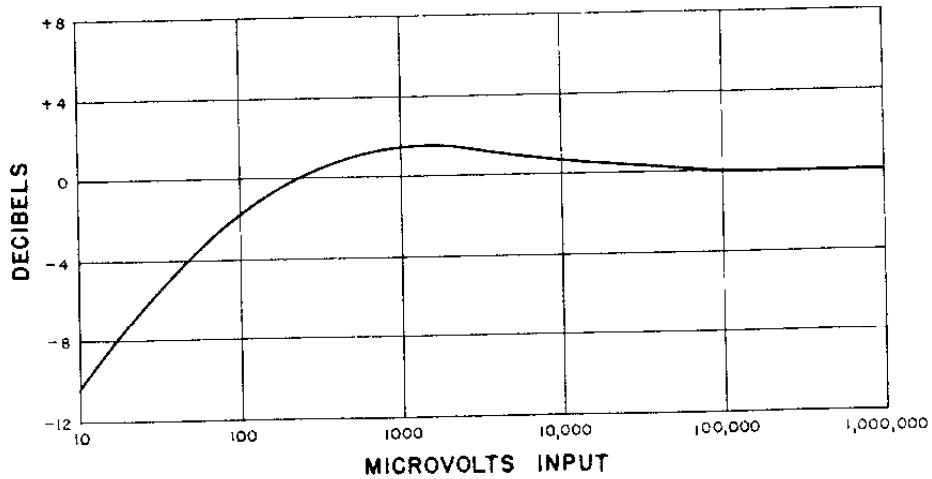
FIG. 7—A.V.C. CURVE—AT 3 MC.
