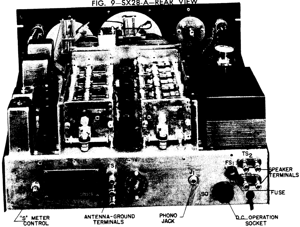
FIG. 9—SX28-A—REAR VIEW
