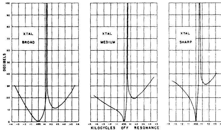
FIG. 4—CRYSTAL SELECTIVITY
